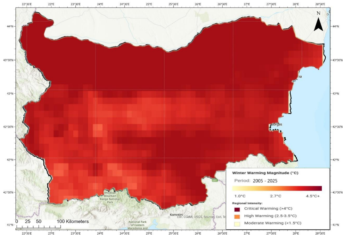
Fig. 13. Spatial distribution of the winter warming magnitude 2005-2025.
