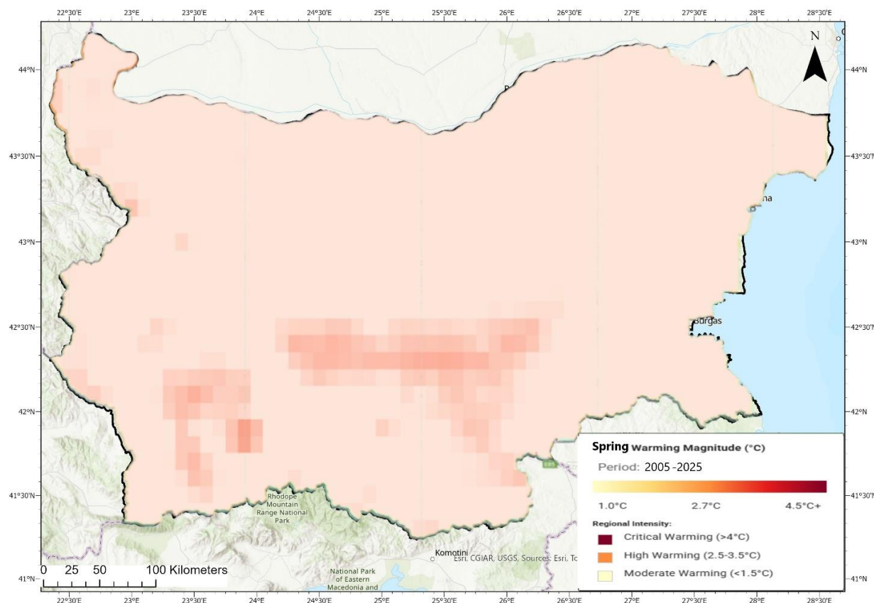
Fig. 16. Spatial distribution of the spring warming magnitude 2005-2025.
