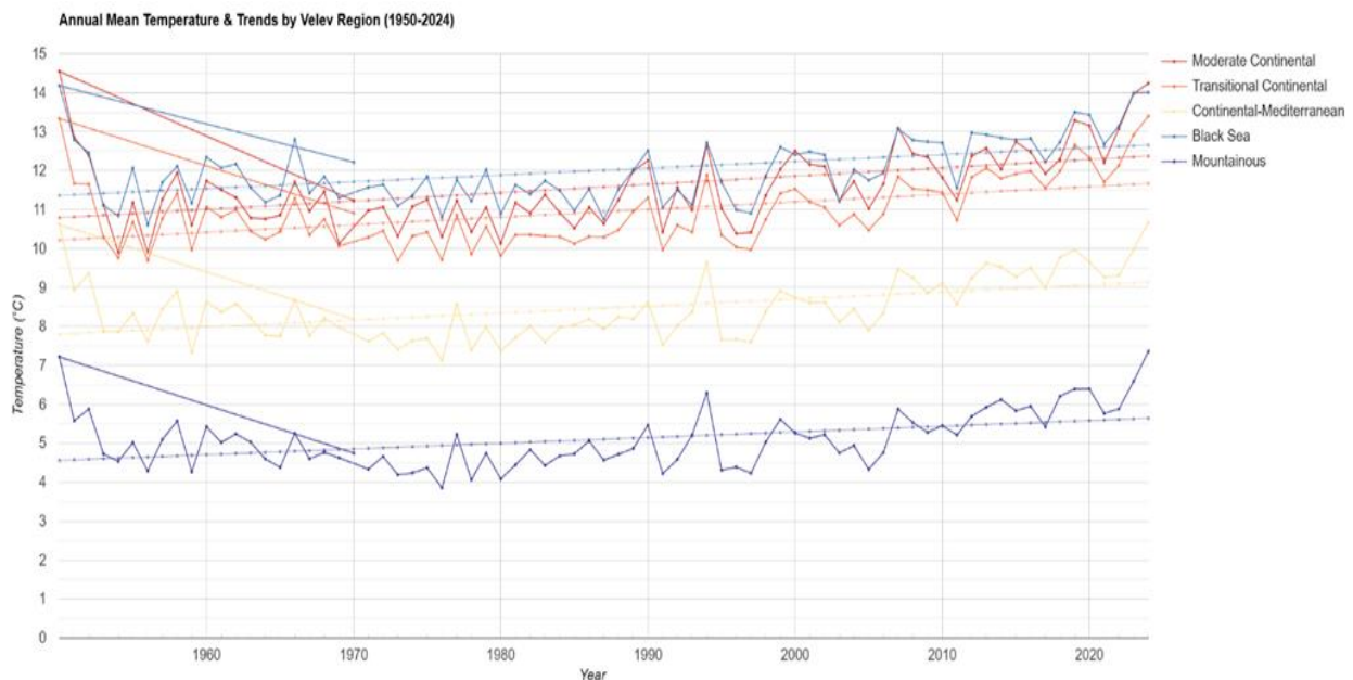
Fig. 3. Dynamics of the mean annual temperatures in Velev (2002) climate regions -1950-2024. Source: Ivanov et al. (2025) .
