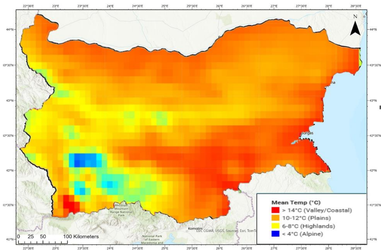
Fig. 1. Spatial distribution of the mean annual temperatures -1950-2024. Source: Ivanov et al. (2025) .
