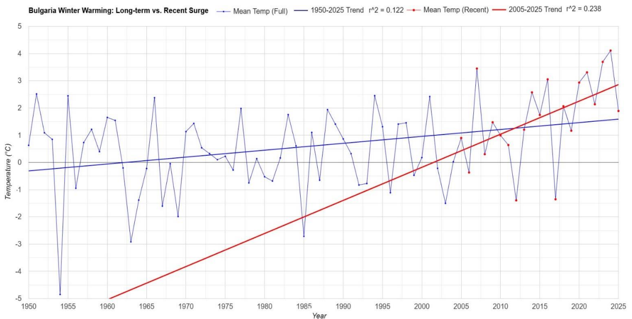
Fig. 11. Winter warming long term vs. recent 20 years.
