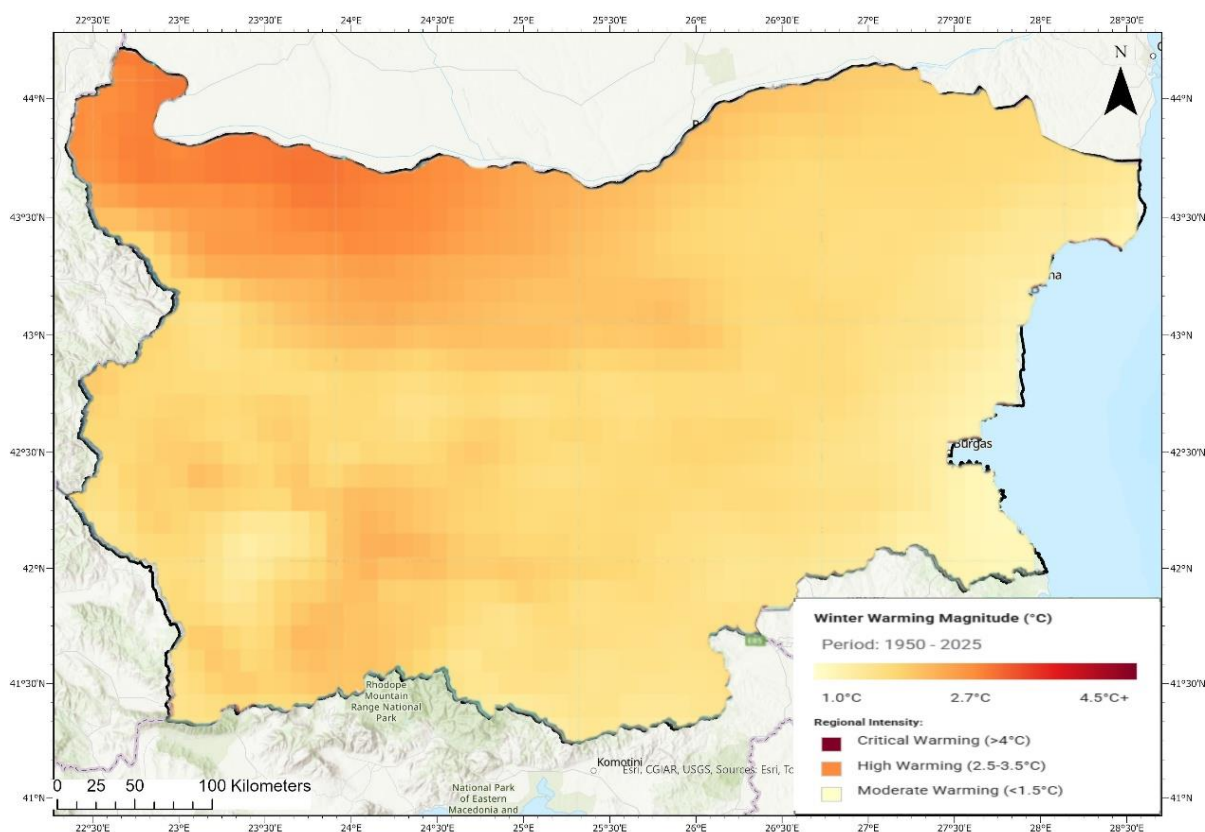
Fig. 12. Spatial distribution of the winter warming magnitude 1950-2025.
